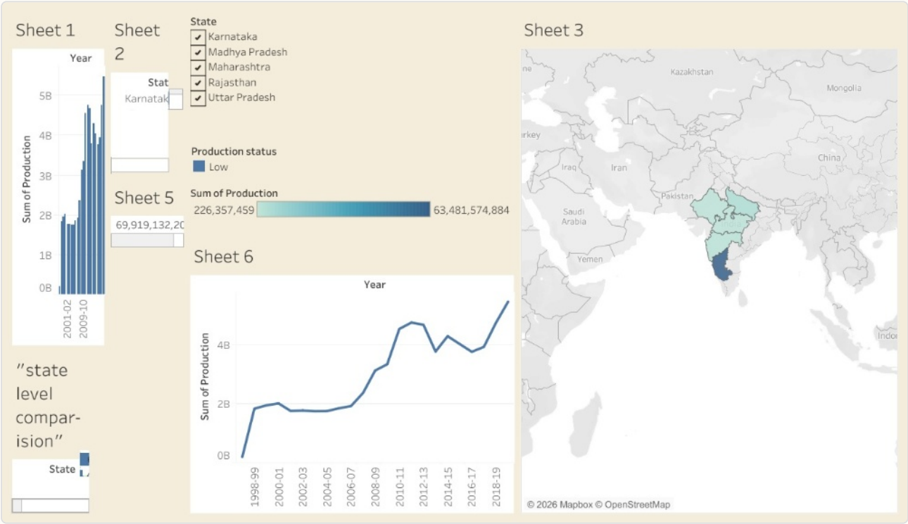
Figure 1: Dashboard Overview
